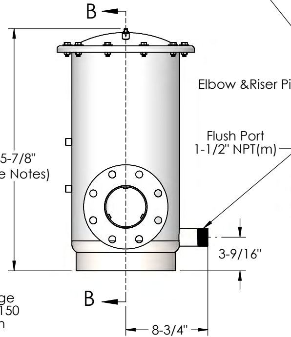
SECTION B-B
