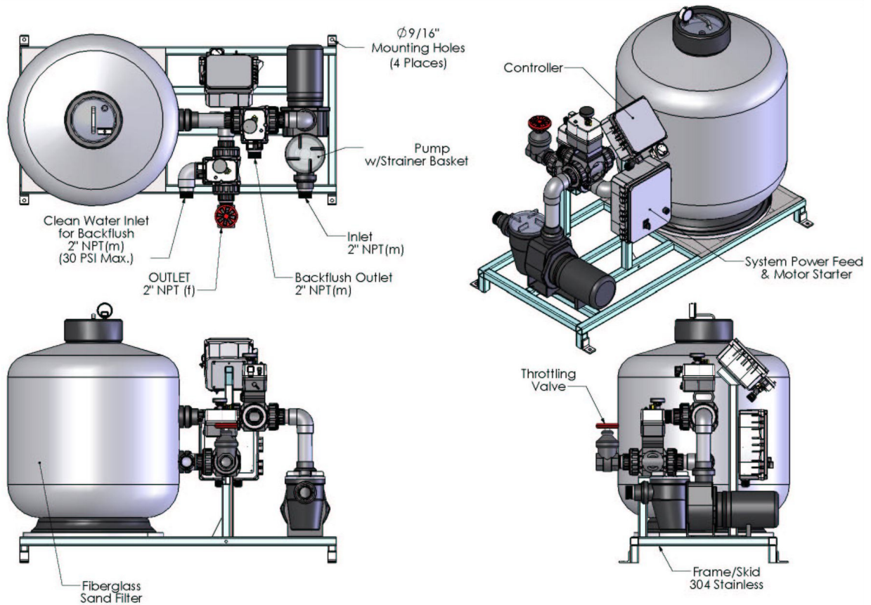
Figure 2. TowerGuard System Layout using the City Water backflush hookup.
