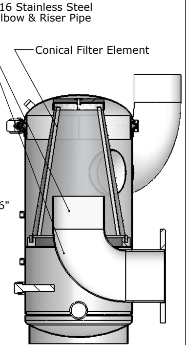
SECTION B-B
